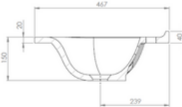
PROFIL VASQUE - BASIN PROFILE
