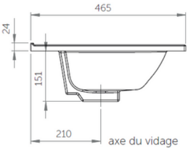
PROFIL VASQUE - BASIN PROFILE
